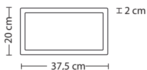
Loxia II - top view
