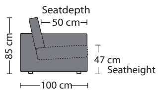
Section 120, 100, 80, 60
