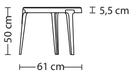
Side table 61 - side view
