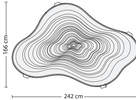
Dining table 242 - top view
