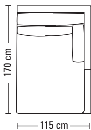
Longchair - top view 1 arm R/L
