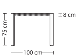
Uluwatu I / Uluwatu I dining table - side view
