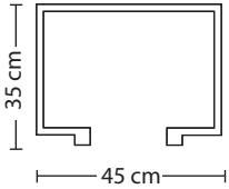
Upsido - side view
